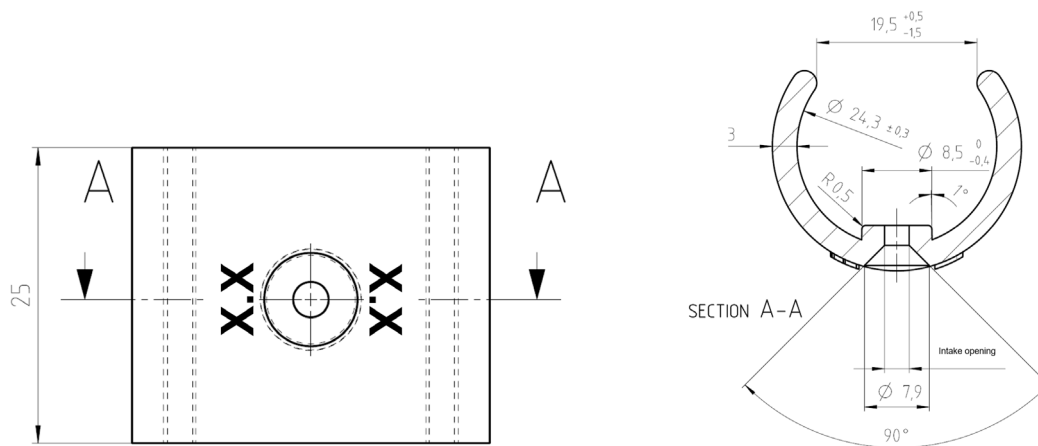
Fig. 3 Drawing sampling clip / maintenance clip PA
