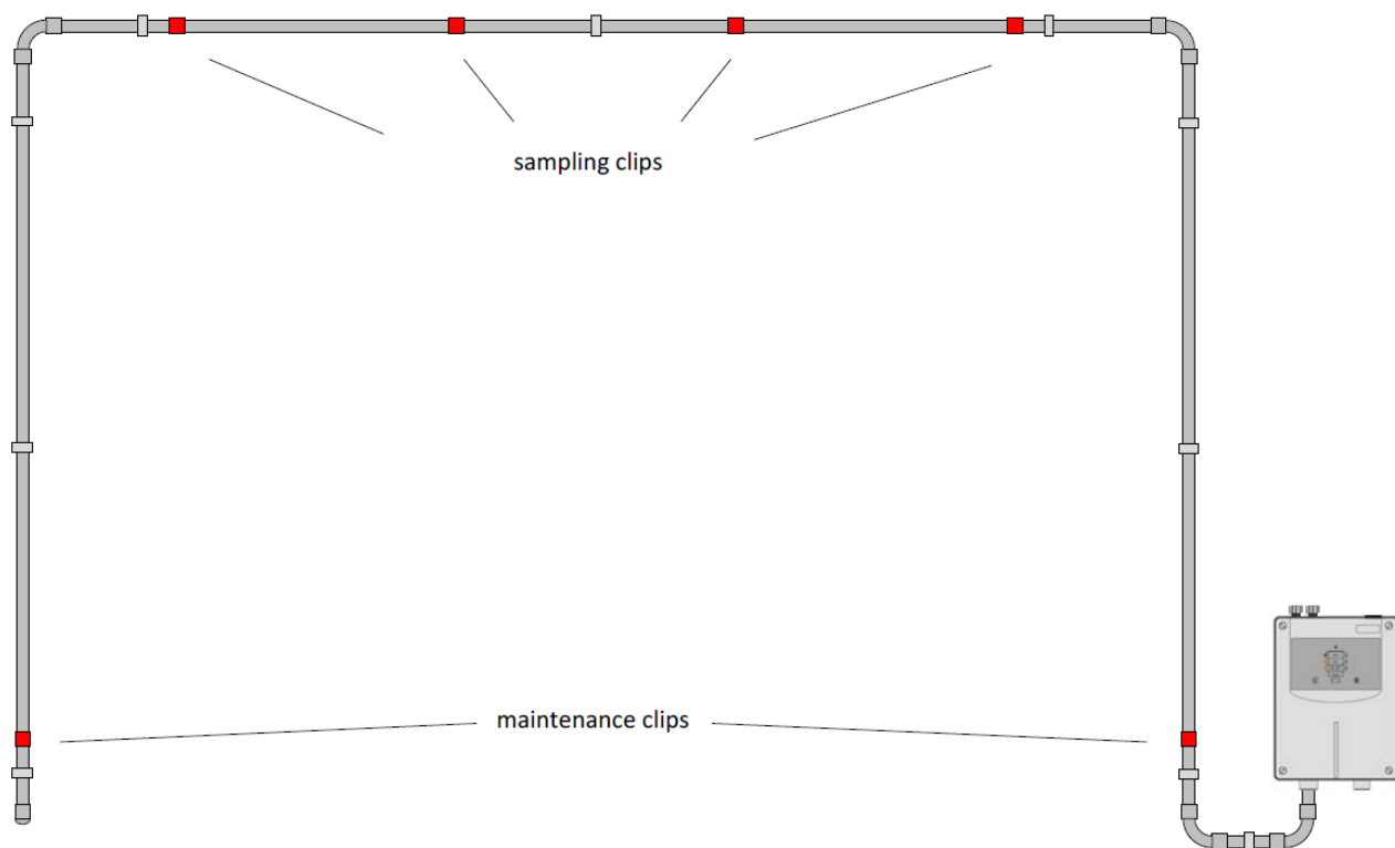
Fig. 2 Possible positions maintenance clip
